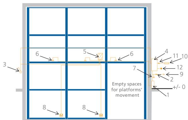
Installation diagram
